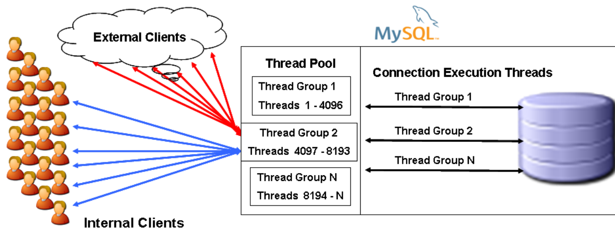
Figure 5: MySQL Thread Pool
