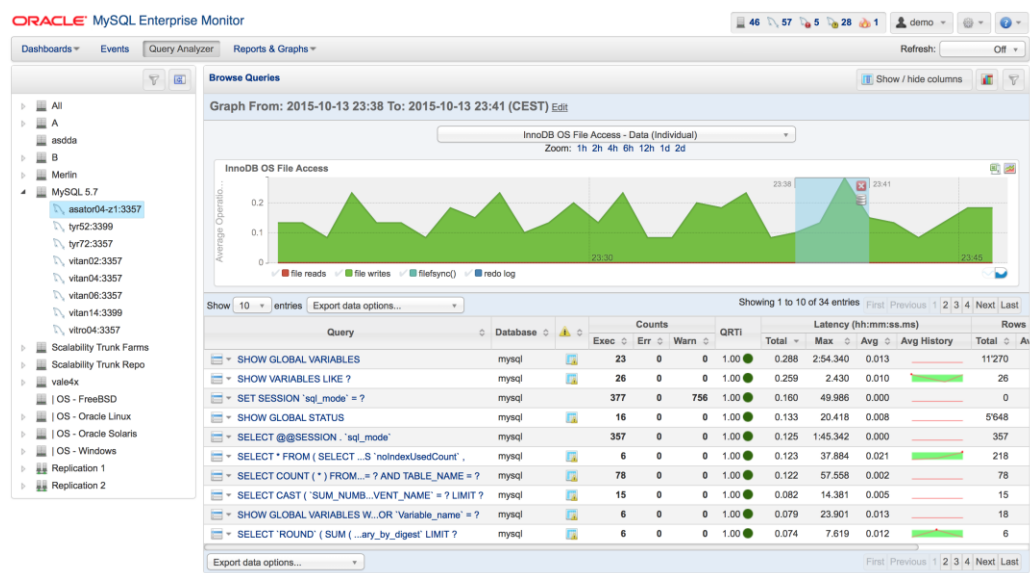
Figure 12: MySQL Query Analyzer
