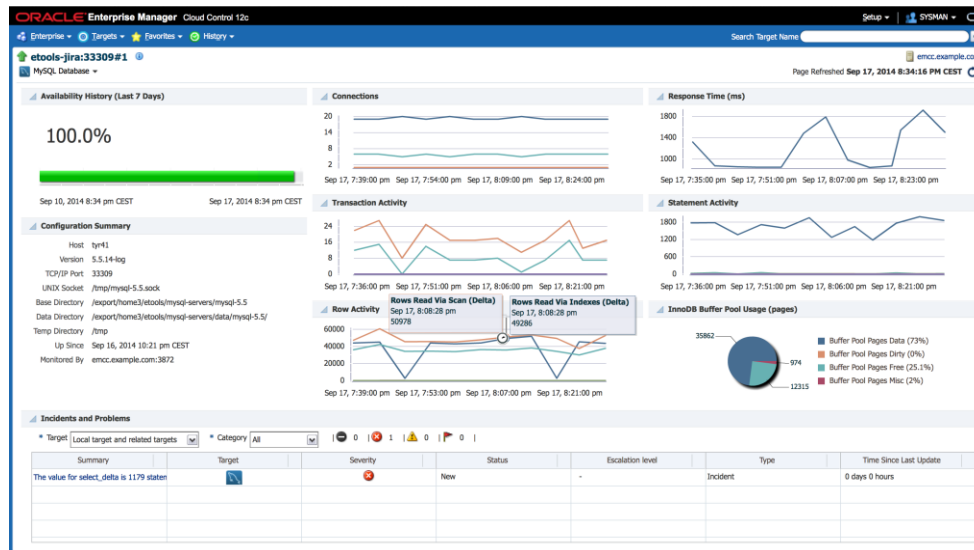
Figure 13: Oracle Enterprise Manager for MySQL allows Oracle developers and DBAs manage MySQL databases.
