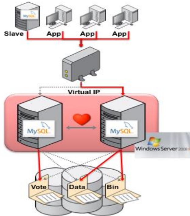
Figure 8: MySQL and Windows Server Failover Cluster Providing HA to Business Critical Applications running on the Windows Platform
