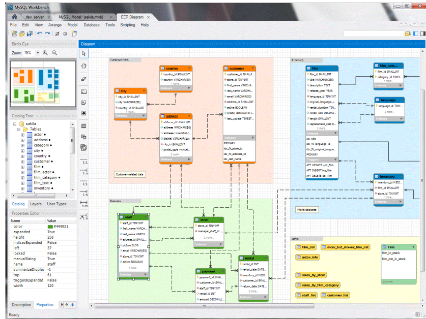
Figure 14: MySQL Workbench – Visual Database Design
