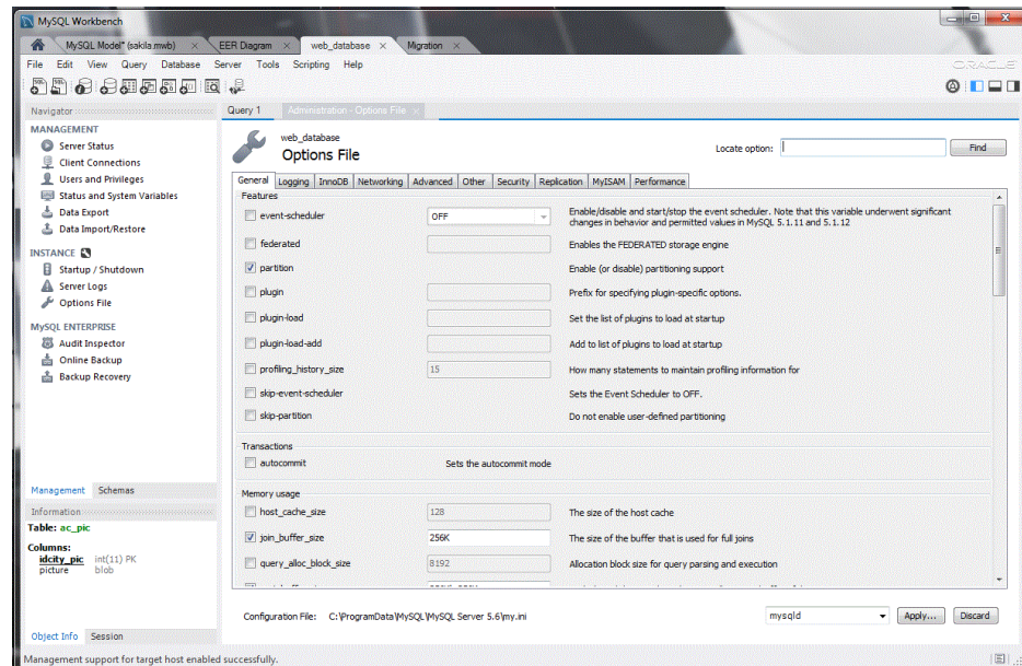
Figure 16: MySQL Workbench – Server Administration, Monitoring
