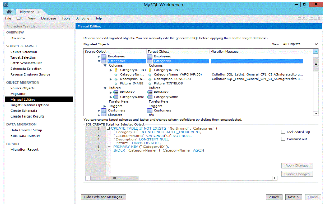
Figure 17: MySQL Workbench – Database Migration Wizard
